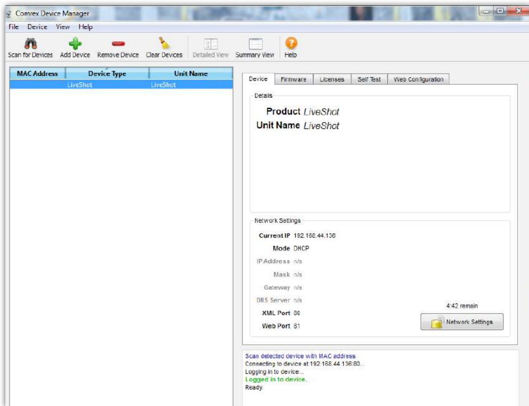
FIGURE 11 DEVICE MANAGER
