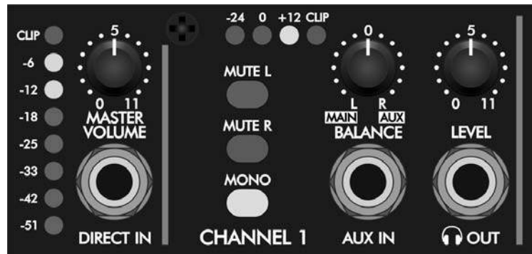
FIGURE 1 - Master Volume, Direct In, and Channel One
