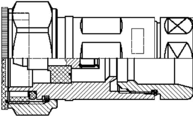
716M-LCF12-C02_CRing.png
